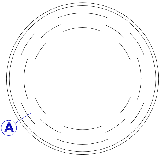
PLAN - CIRCLE SKYLIGHT NTS
